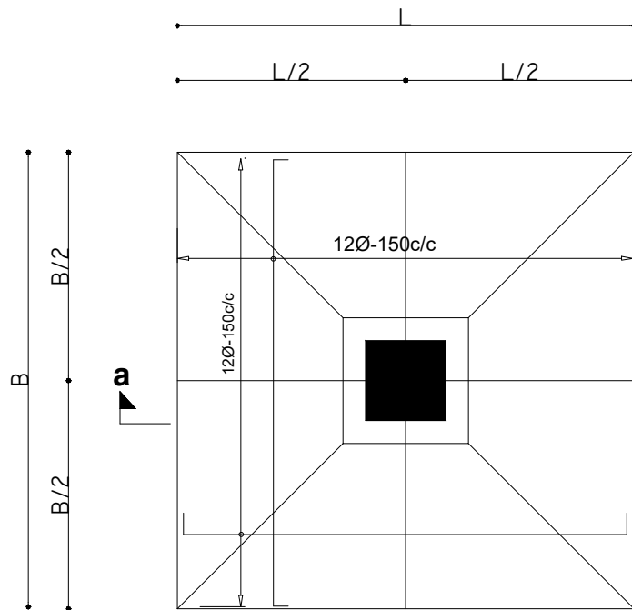
ISOLATED FOOTING PLAN
