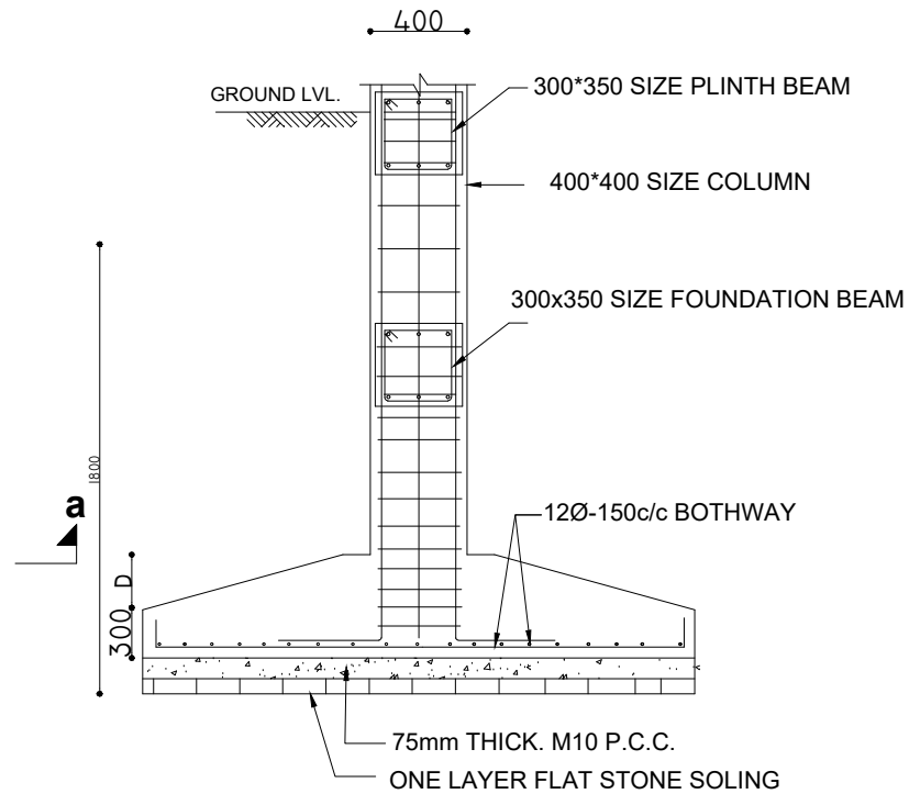
MAIN GATE FOOTING SECTION
