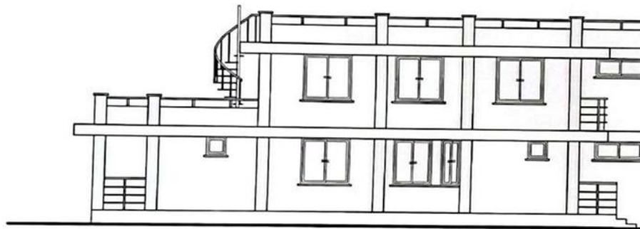
BACK ELEVATION
